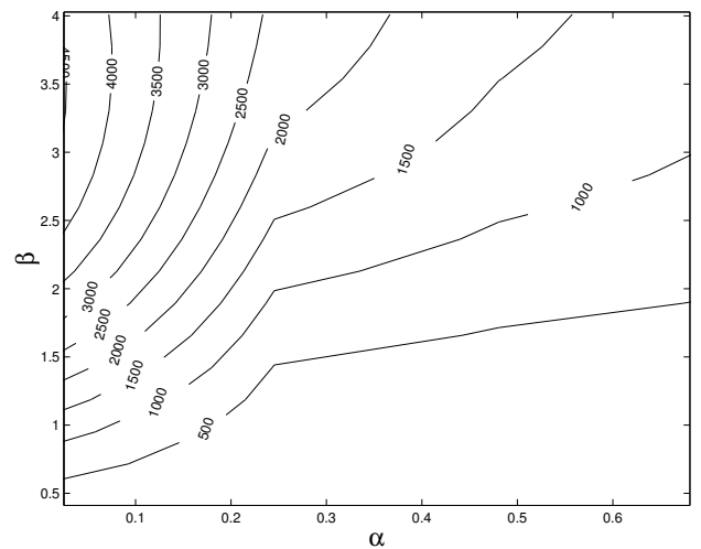
Figure 2: Maximum amplification factors G_{MAX} of three-dimensional disturbances in two-phase shear flow with r = 10^{-2}, m = 10^{-2}, We = 100 and Re = 100 .
