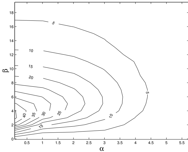
Figure 1: Maximum amplification factors G_{MAX} of three-dimensional disturbances in two-phase shear flow with r = 10^{-1}, m = 10^{-2}, We = 100 and Re = 100 .
